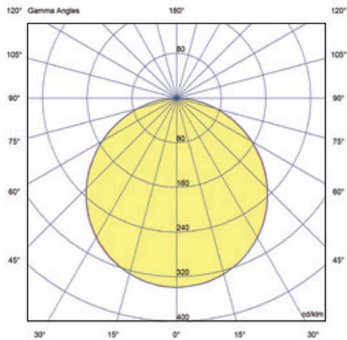
Polar Curve: ECOPL123CSEG2
