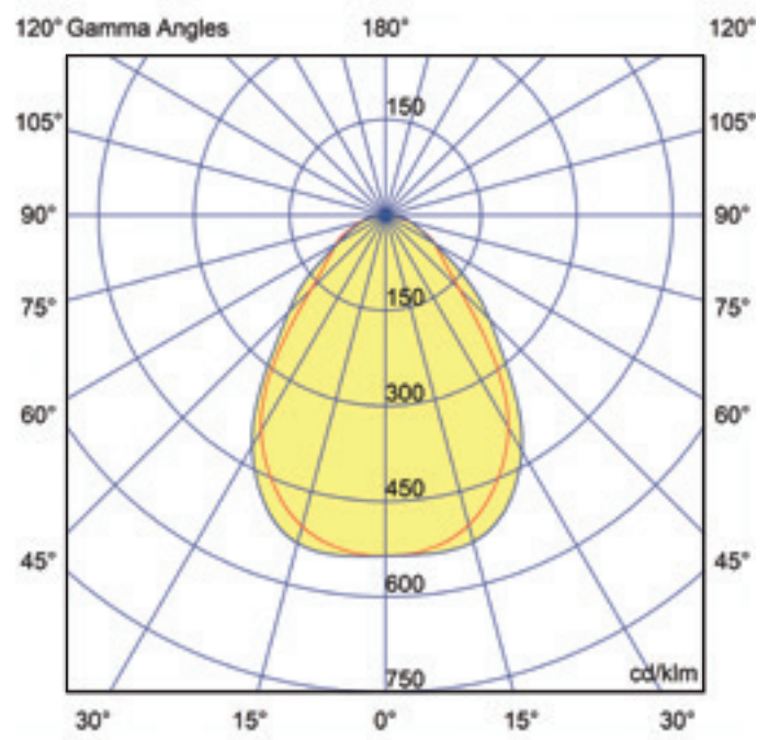
Polar Curve: SL123CK19D1
