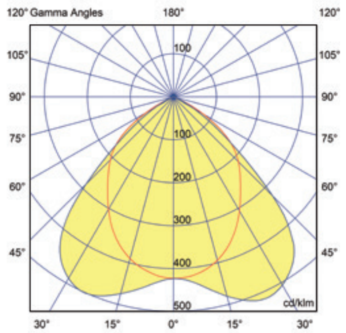
Polar Curve: FLED2B12349D4
