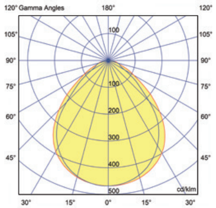
Polar Curve: DLED3R12349D4
